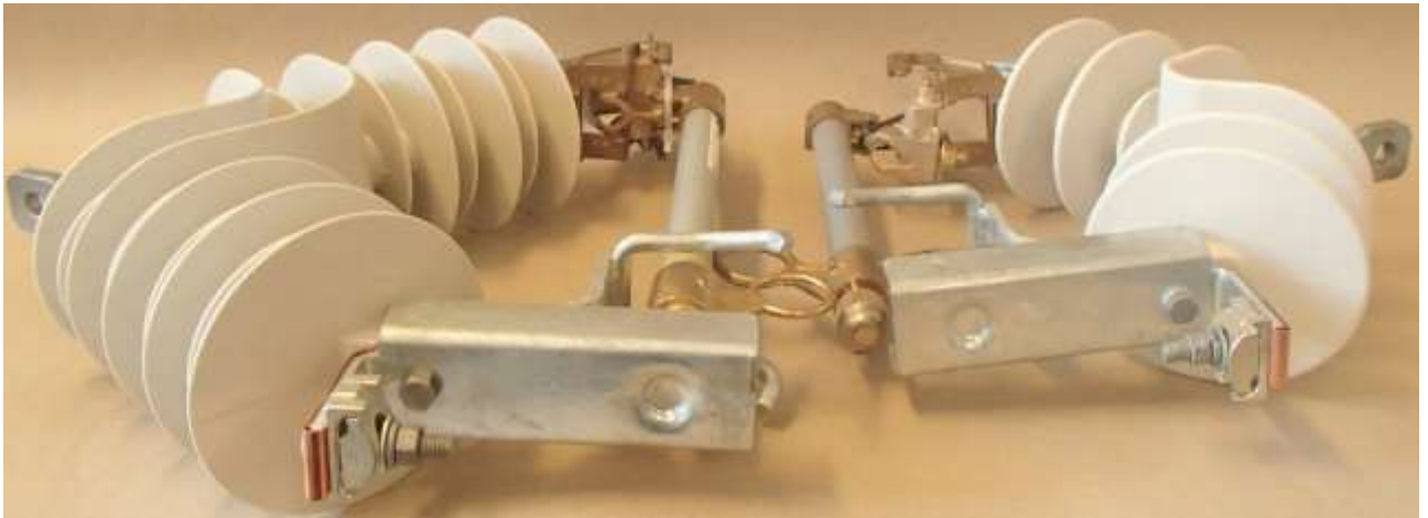
COI 15kV & 27 kV (View 2)
